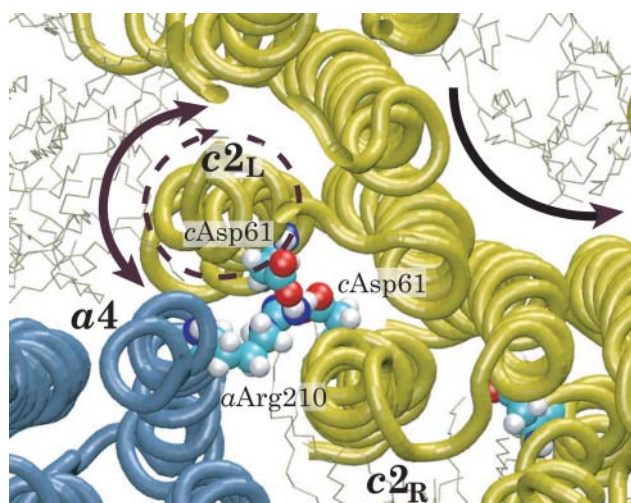
FIGURE 8 Concerted rotation of the c -subunit outer helix and the c_{10} complex in a lipid bilayer. The c_{2L} helix has been forced to rotate clockwise by 180^\circ . Shown in the instance when the salt bridge is transferred between two neighboring c -subunits, i.e., when the conformation cAsp-61^- - aArg-210 - cAsp-61^- has been momentarily assumed.
