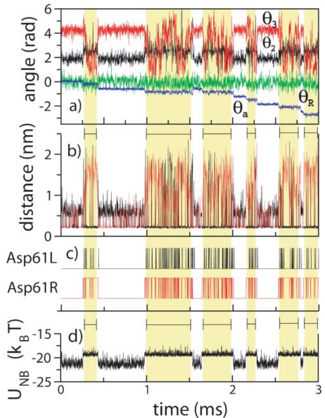
FIGURE 9 Stochastic events involved in F o function. (a) Time evolution of helix angles \theta_2 (black), \theta_3 (red), \theta_R (green), and rotor angle \theta_a (blue). The angles are defined in Fig. 4. The a -subunit rotation takes place in discrete steps (blue line). (b) Distances between residues a Arg-210– c Asp-61 of c 2 L (black) and a Arg-210– c Asp-61 of c 2 R (red). Respective salt bridges are formed when these distances decrease below \sim 0.25 nm. When both aspartates are deprotonated, a two-color pattern of lines at 0.25 nm indicates a frequent transfer of the salt bridge from one aspartate to another. When one of the aspartates is protonated (highlighted regions), a two-color pattern does not indicate a salt bridge transfer, but originates from the cyclic boundary conditions invoked when subunit a passes the boundary. (c) Protonation states of c Asp-61L (black) and c Asp-61R (red) (see text). (d) Nonbonded interaction energy of the three residues. The steps of the energy function are correlated with protonation/deprotonation of two c Asp-61 residues and the step motion of the a -subunit.
