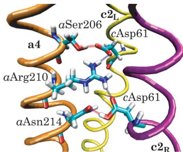
FIGURE 7 Hydrogen-bond network formed between the binding sites ( cAsp-61 ) and the terminal residues of the proton periplasm ( aAsn-214 ) and cytoplasm ( aSer-206 ) channels. The critical residue aArg-210 forms transient hydrogen bonds with both binding sites.
