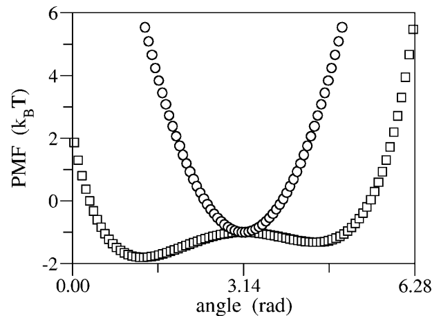
FIGURE 5 Potentials of mean force used in the stochastic simulations: a double-well potential governing rotation of the c2 helices (open squares) and a parabolic potential governing rotation of the a4 helix (open circles).
